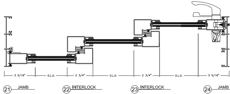
HORIZONTAL SECTIONS
