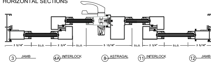
HORIZONTAL SECTIONS
