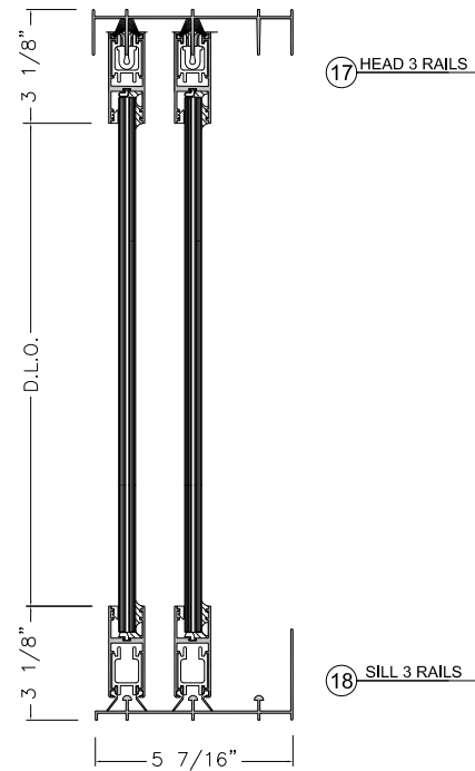
VERTICAL SECTIONS
