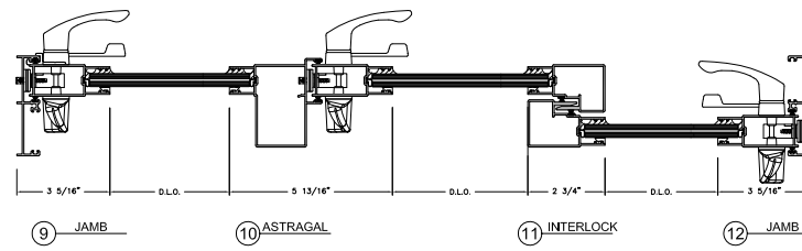
HORIZONTAL SECTIONS
