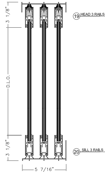
VERTICAL SECTIONS
