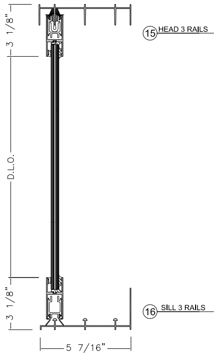
VERTICAL SECTIONS
